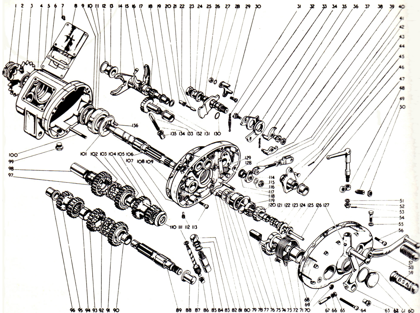
Fig. 2.2. M Series gearbox - component parts
