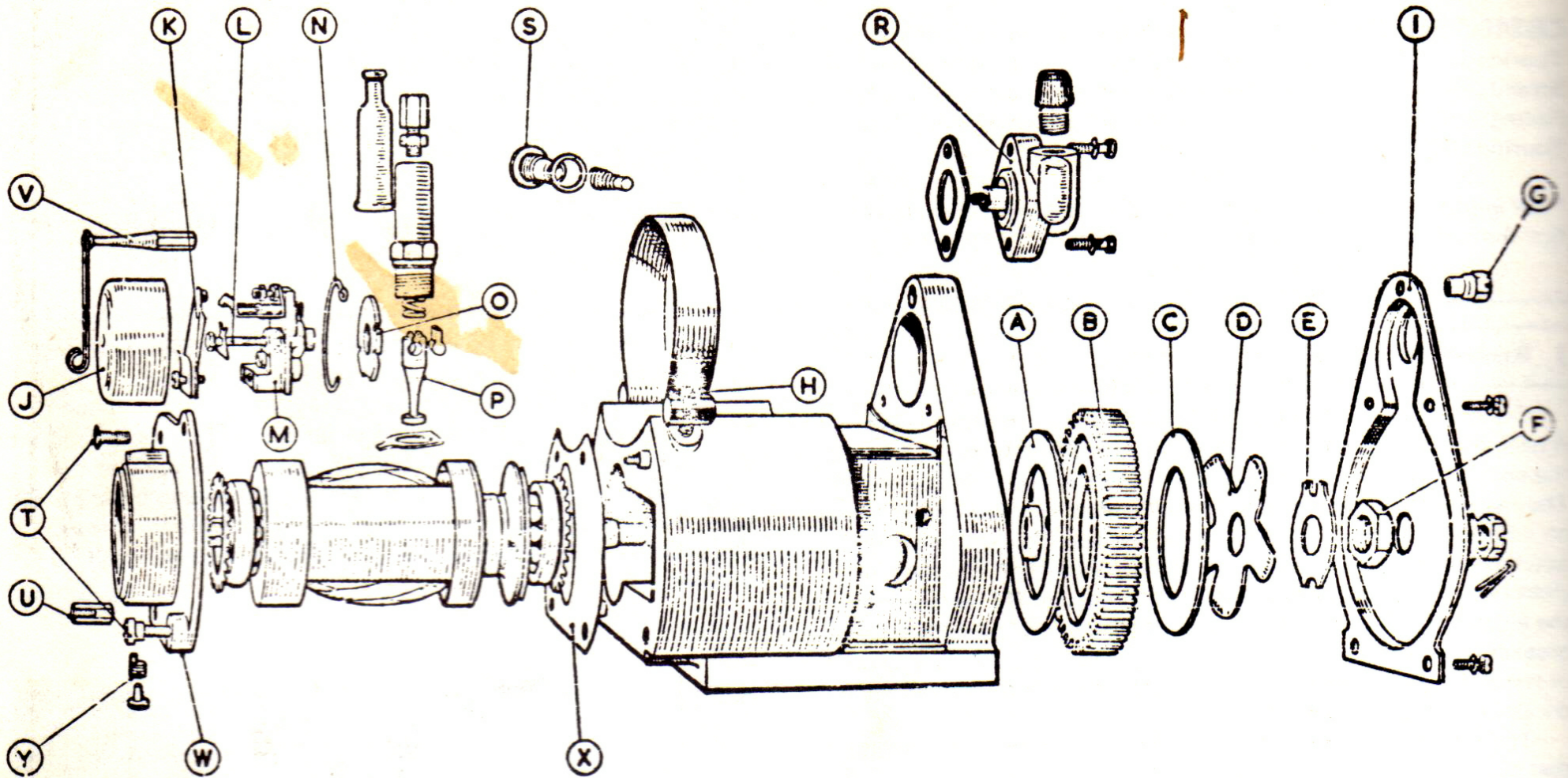
Fig. 5.1. Exploded view of typical single-cylinder Magdyno
