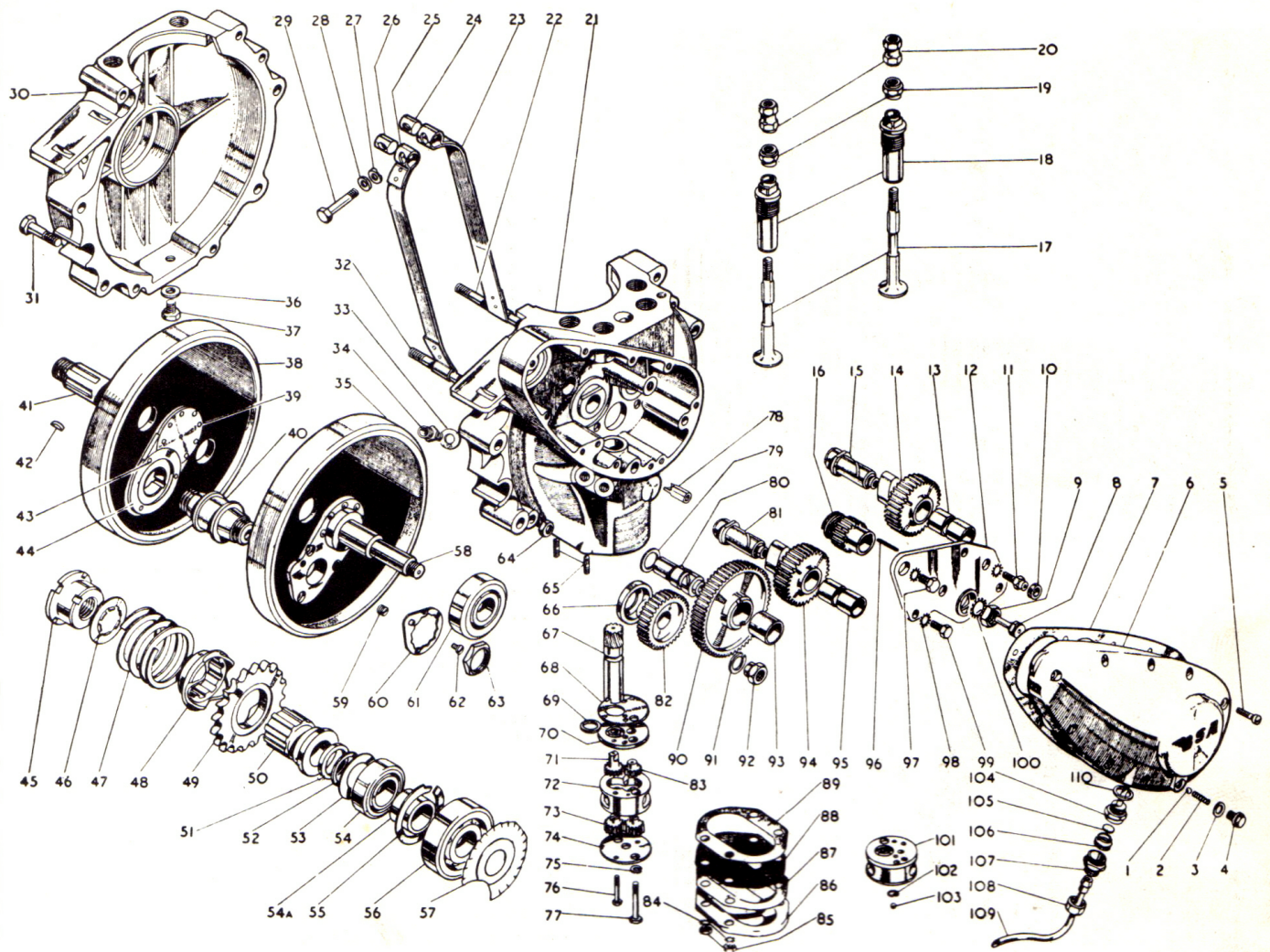
Fig. 1.5. Crankcase assembly - except Gold Star models - component parts
